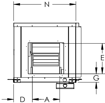
END DISCHARGE VIEW
