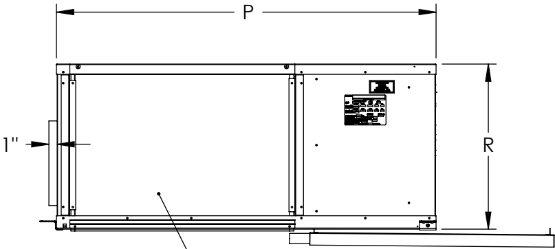
RETURN AIR-FILTER
