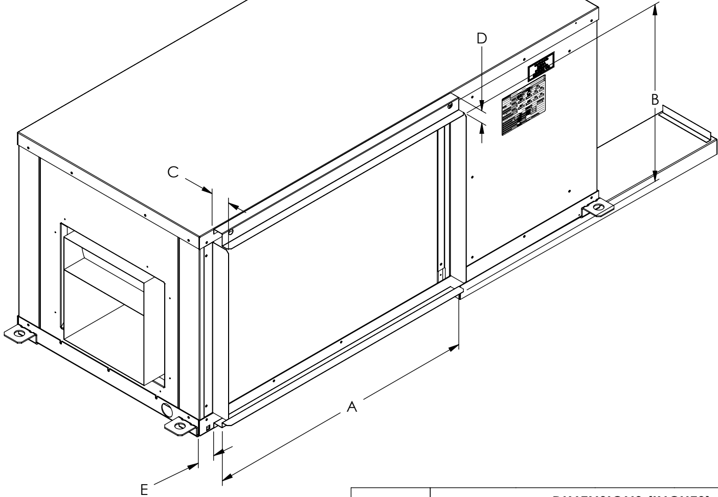
LEFT HAND RETURN, END DISCHARGE
